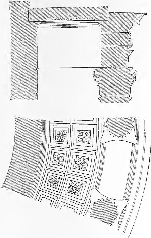
FIG. 122.—THE TEMPLE OF VESTA AT TIVOLI. PLAN (LOOKING UP) AND SECTION OF PART OF THE PERISTYLE.
